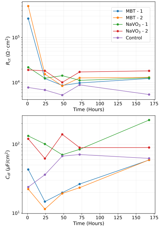
Figure 3: Evolution of R_{ct} and C_{dl} over the 168 h immersion period for the LDH-2 specimens.
