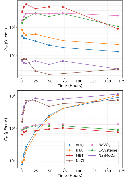
Figure 1: Evolution of R_{ct} and C_{dl} over the 168 h immersion period for the pre-selected inhibitors.
