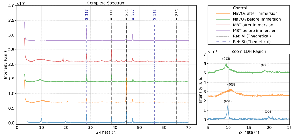
Figure 2: XRD patterns of LDH films in the nitrate form (control), following \text{NaVO}_3 intercalation, and following the MBT intercalation attempt, each presented before and after immersion in 0.05 M NaCl.
