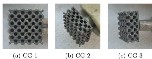
Figure 4: Optical macrographs of polyurethane-coated complex-shaped specimens.
